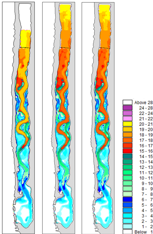
Local water renewal times in days for actual conditions (left), proposed removal of upstream dike (center) and proposed dredging of flood delta circulation channels (right) © DHI / Hydrosoft S.A.
